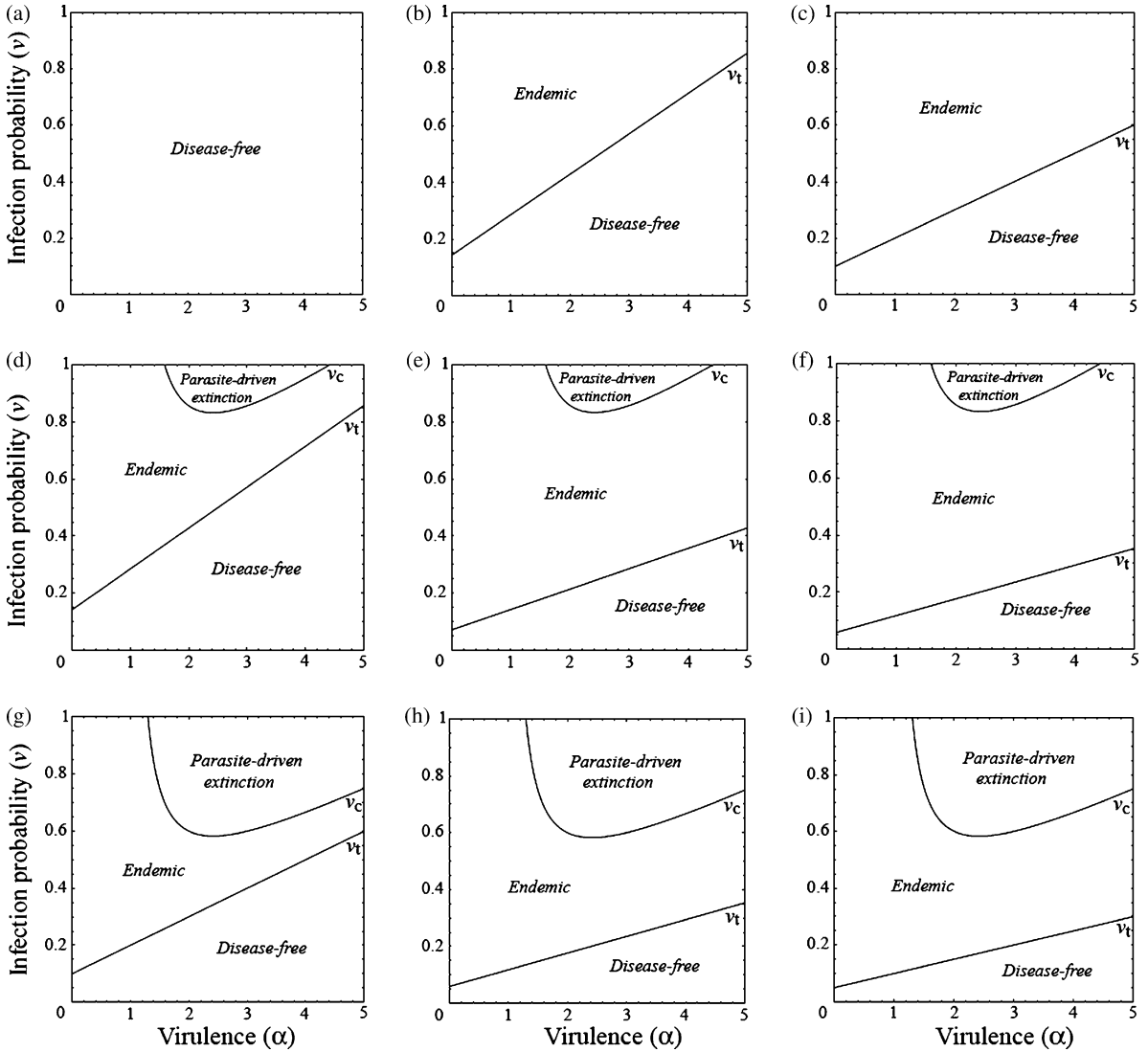
Fig. 1. Outcomes in (v, \alpha) parameter space for different levels of frequency- and density-dependence: (a) m=0, c=0 ; (b) m=7, c=0 ; (c) m=10, c=0 ; (d) m=0, c=7 ; (e) m=7, c=7 ; (f) m=10, c=7 ; (g) m=0, c=10 ; (h) m=7, c=10 ; (i) m=10, c=10 . The other parameters are: b=2, u=1 and h=1 . The carrying capacity is N_K=1 .
